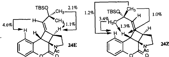
NOE Data for 24E and 24Z .
